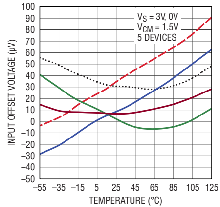
V_{OS} vs Temperature, 3V Supply
