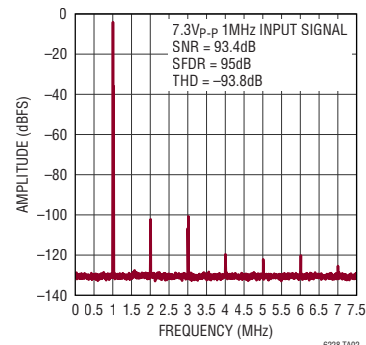
System Performance: 2 x LTC6228 Driving LTC2387-18 8192 Point FFT, -1dBFS f SAMPL = 15Mps, f IN = 1MHz
