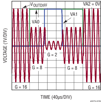
Gain Switching Transient Response
