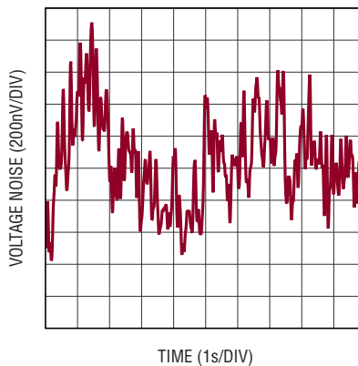
Input Referred 0.1Hz to 10Hz Voltage Noise (G = 2)
