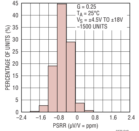
Typical Distribution of Differential PSRR
