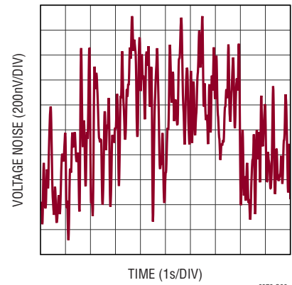
Input Referred 0.1Hz to 10Hz Voltage Noise (G = 1)
