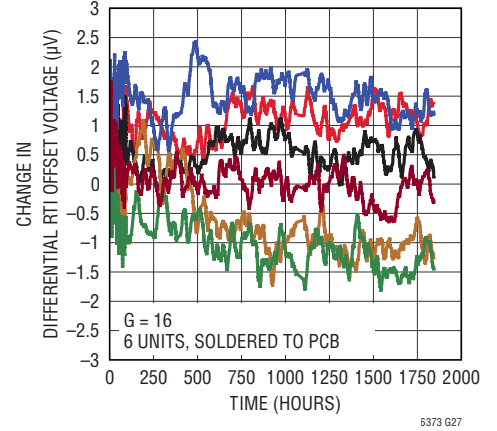
Long Term Differential RTI Offset Voltage Drift
