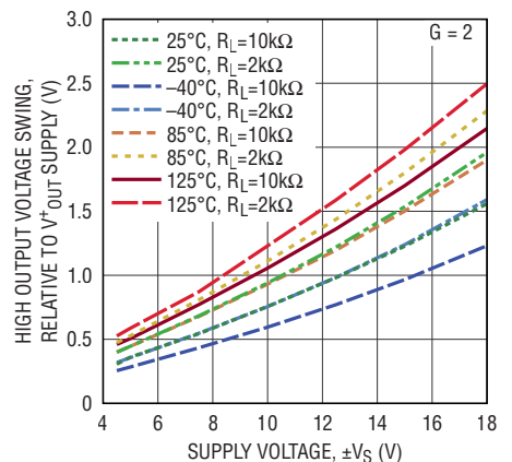
High Output Voltage Swing vs Supply Voltage
