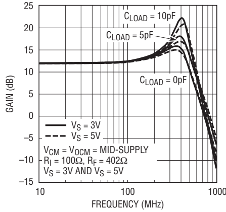
Small-Signal Frequency Response vs C_{LOAD}
