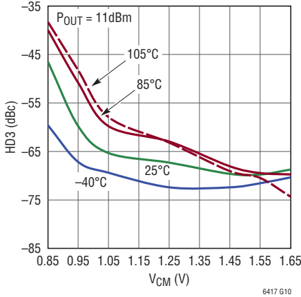
HD3 at 240MHz vs V_{CM} Over Temperature
