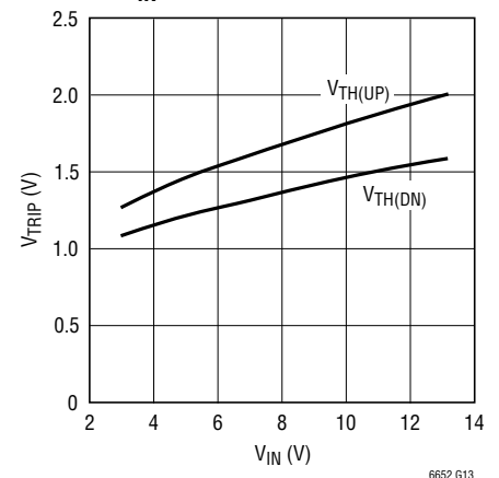
\overline{\text{SHDN}} Input Voltage Thresholds vs V_{\text{IN}}
