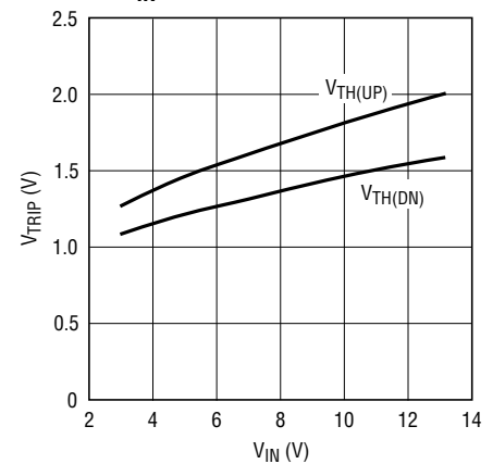
\overline{SHDN} Input Voltage Thresholds vs V_{IN}
