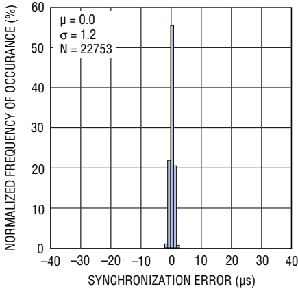
TIMEn Synchronization Error 1 Packet/s Publishing Rate, 1 Hop, Room Temperature
