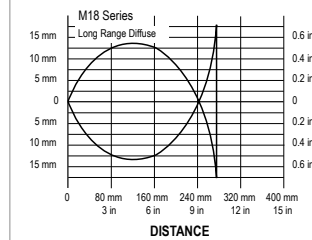
Beam Pattern
