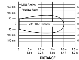
Beam Pattern
