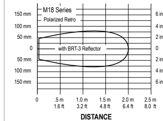
Beam Pattern
