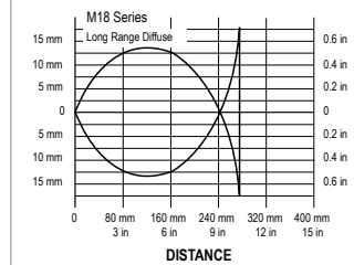
Beam Pattern
