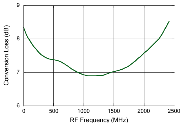
Conversion Loss
