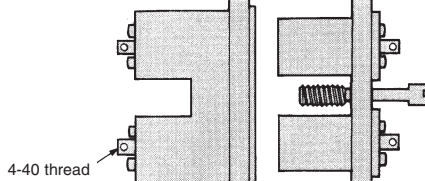
Modification 52 (R, RM, M, MM—attaching tabs)
