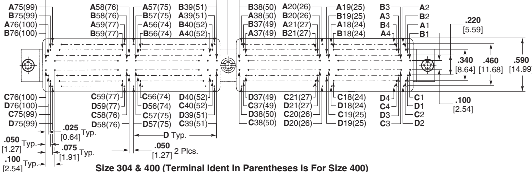
Size 304 & 400 (Terminal Ident In Parentheses Is For Size 400)
