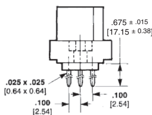
Solder Eyelet Contact
