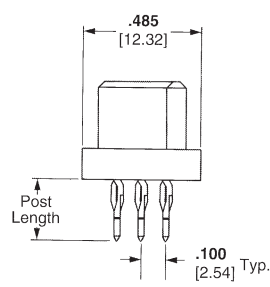
ACTION PIN Posts
