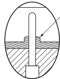
Interfacial Seal (unbonded) Mat'l: Fluorosilicone
