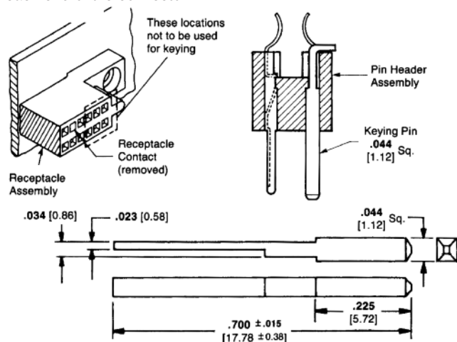
Material: Nickel plated brass Part Number 530328-2 Military Part Number M55302/31-03
