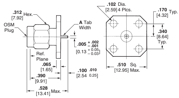
Outline 4
