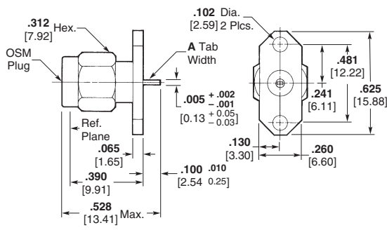
Outline 3
