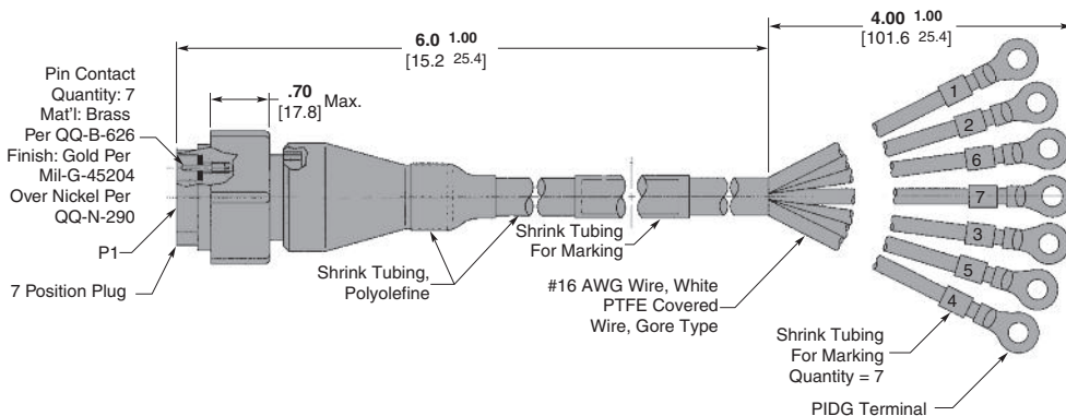
Part Number 447288-1
