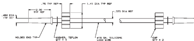
Part Number 445217
