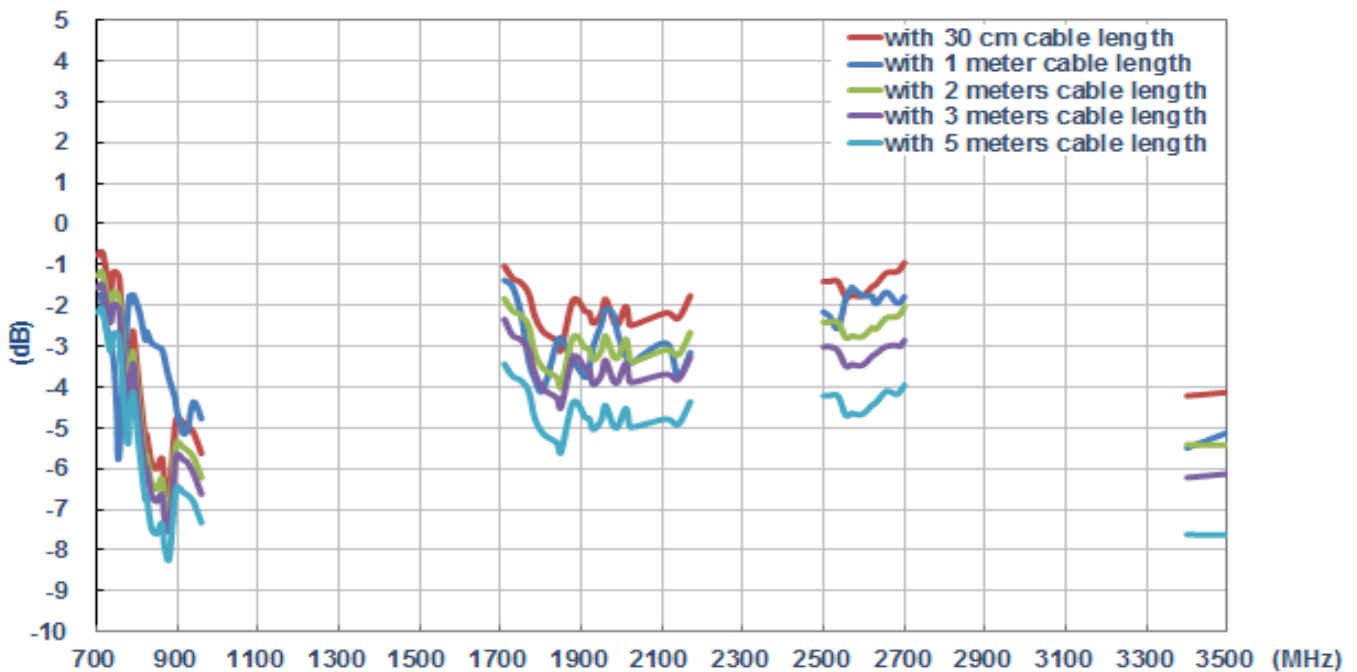
Average Gain (ANTENNA_1 on glass)
