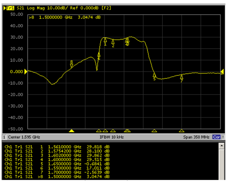
LNA Gain and Out Band Rejection @3.0V
