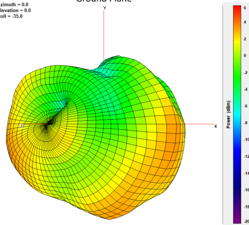
MIMO 2 – 30cmx30cm Ground Plane Azimuth = 0.0 Elevation = 0.0 Roll = -35.0
