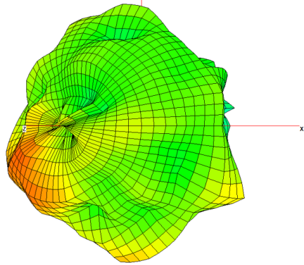
MIMO 1 – 30cmx30cm Ground Plane
