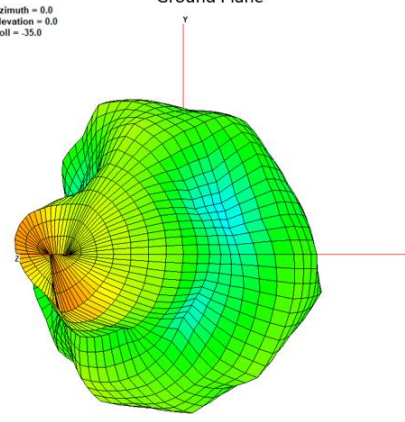
MIMO 2 – 30cmx30cm Ground Plane
