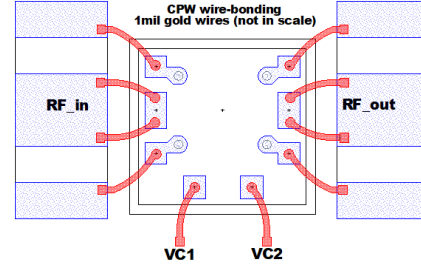
(b) Recommended CPW wire bonding
