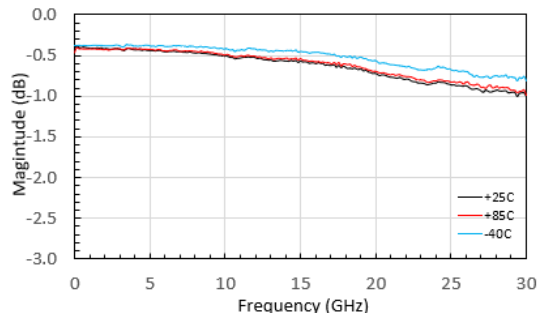
Insertion Loss, over temperature
