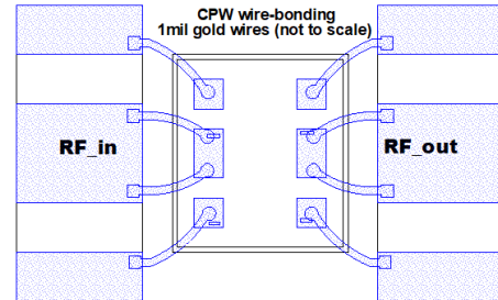
(b) Recommended CPW wire bonding
