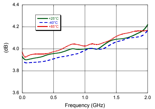
Attenuation @ 16 dB
