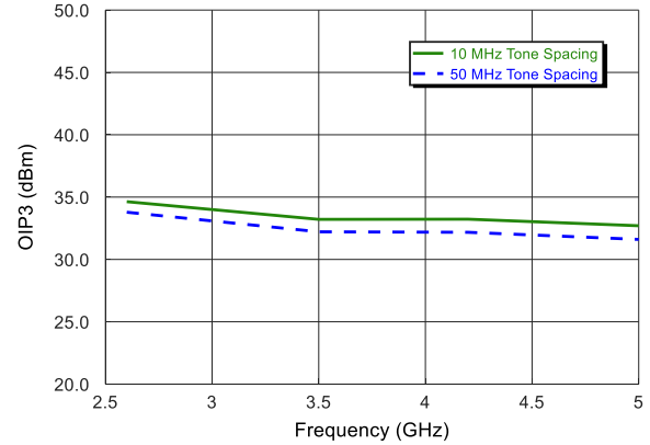
Channel B OIP3 over swept frequency. P_{OUT}/\text{Tone} = 6 \text{ dBm} with 10 MHz & 50 MHz tone spacing in HGM.
