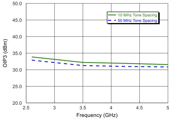
Channel A OIP3 over swept frequency. P_{OUT}/\text{Tone} = 6 \text{ dBm} with 10 MHz & 50 MHz tone spacing in HGM.
