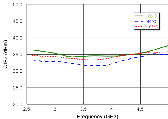
Channel B OIP3 over swept Frequency (& Temp.) with P_{OUT}/\text{Tone} = 3 \text{ dBm} & 10 MHz tone spacing in HGM.
