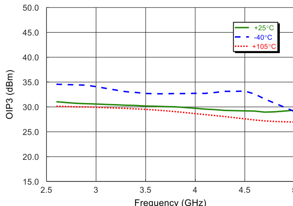
Channel B OIP3 over swept Frequency (& Temp.) with P_{OUT}/\text{Tone} = 3 \text{ dBm} & 10 MHz tone spacing in LGM.
