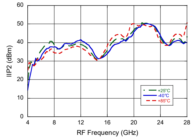
IIP2 over temperature
