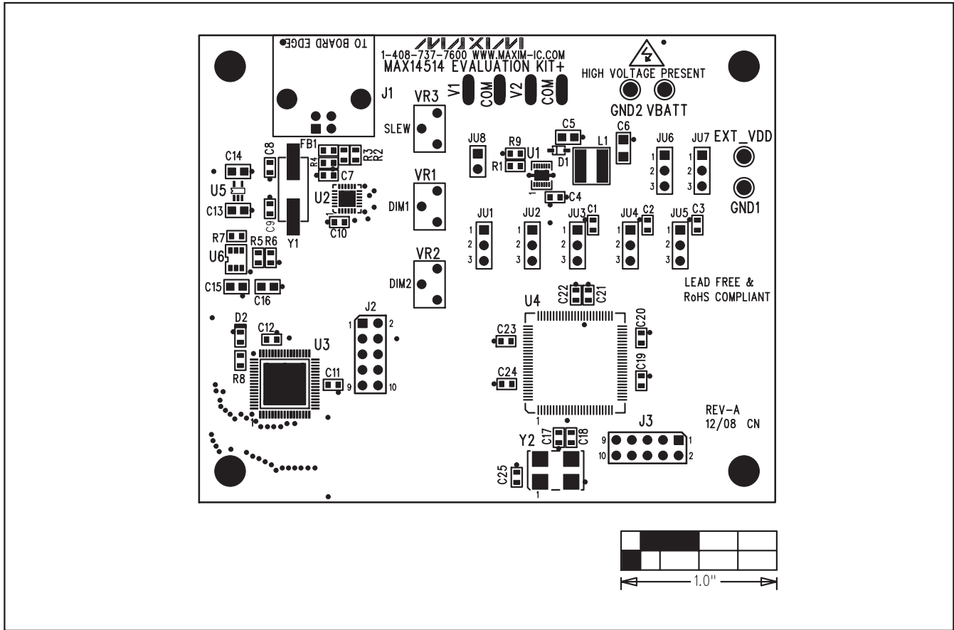
Figure 3. MAX14514 EV Kit Component Placement Guide—Component Side
