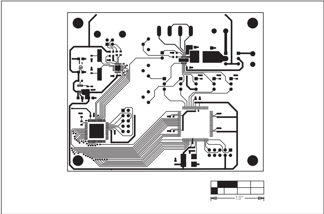
Figure 4. MAX14514 EV Kit PCB Layout—Component Side
