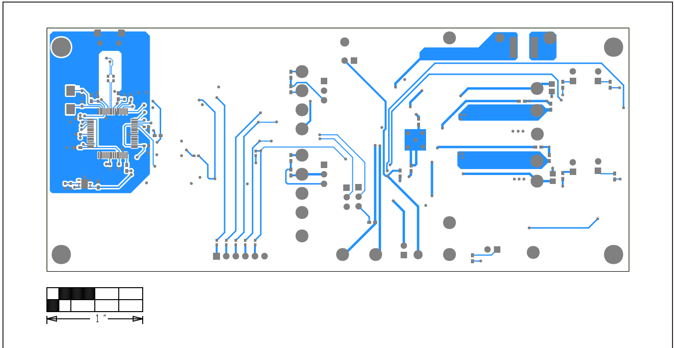
MAX14819 EV Kit—Bottom
