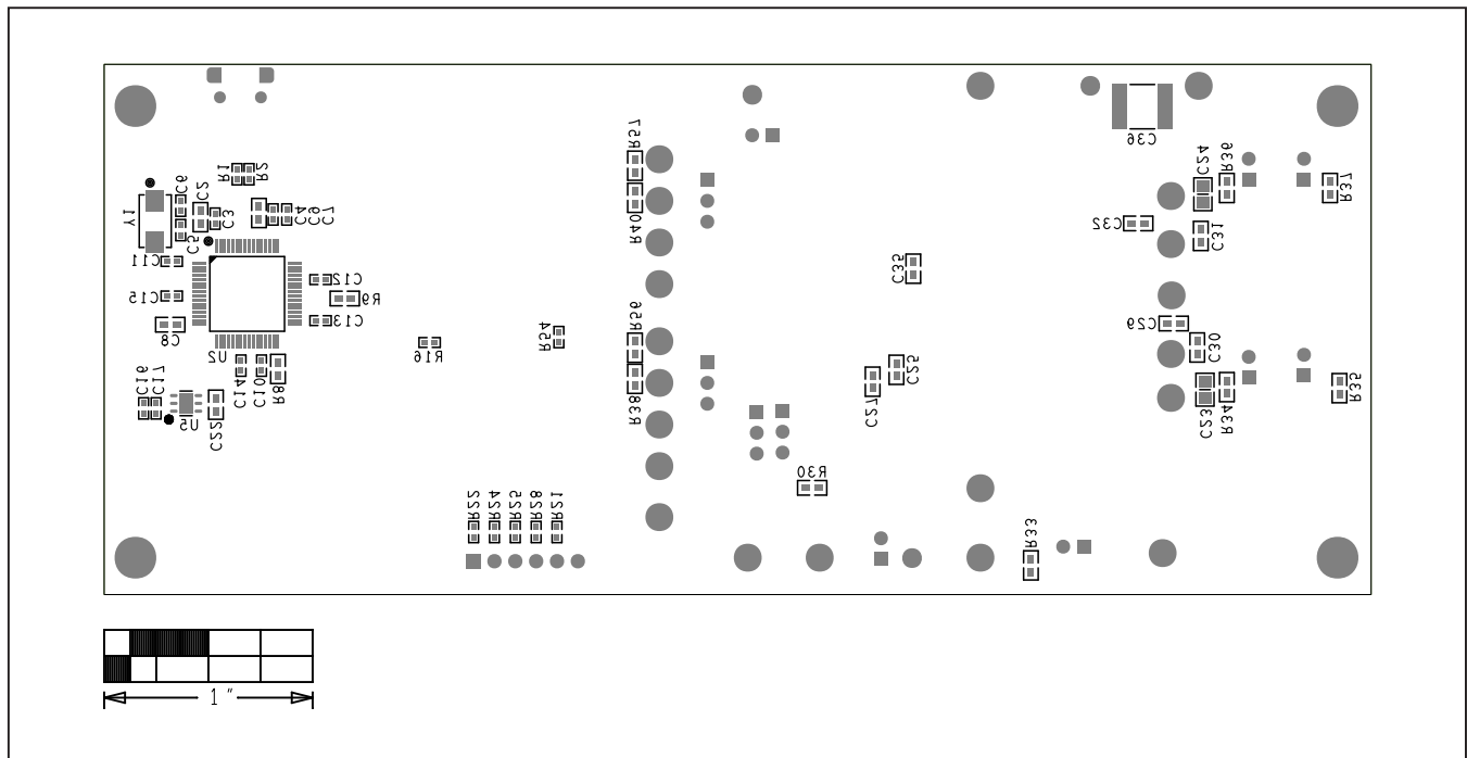
MAX14819 EV Kit—Bottom Silkscreen
