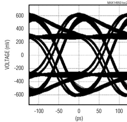
INEQ0 = INEQ1 = 0, V_{IN} = 200\text{mVp-p} , OEQ2 = 0, OEQ1 = 1, OEQ0 = 1, DATA RATE = 8GT/s
