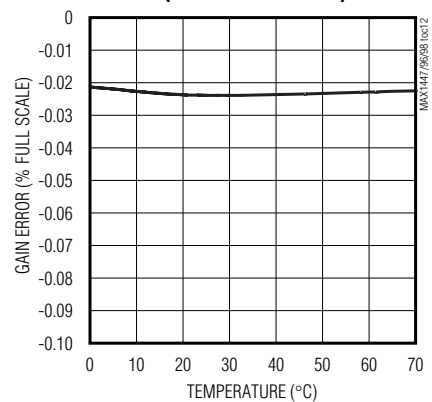
GAIN ERROR vs. TEMPERATURE (MAX1447/MAX1498)
