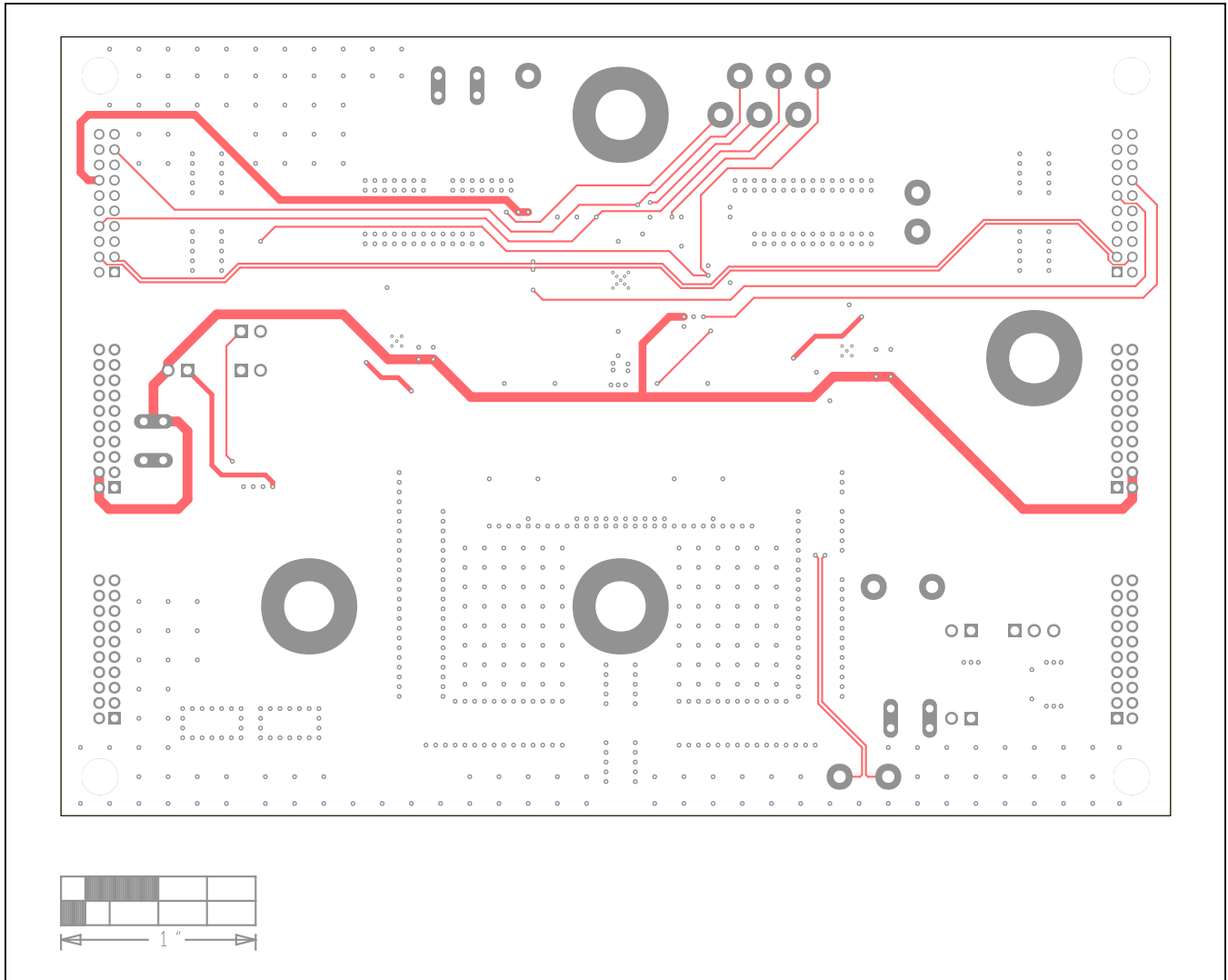
MAX15158Z EV Kit PCB Layout—Internal Layer 4
