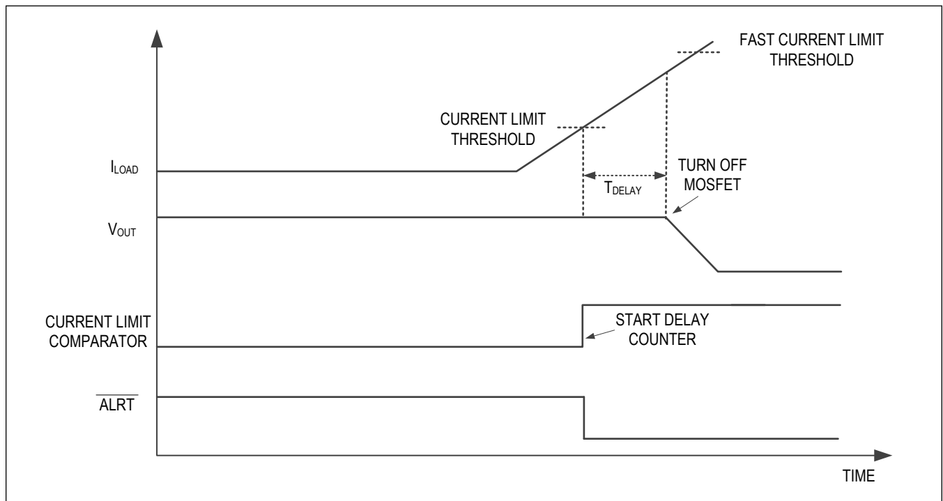
Figure 2. Overcurrent Event
