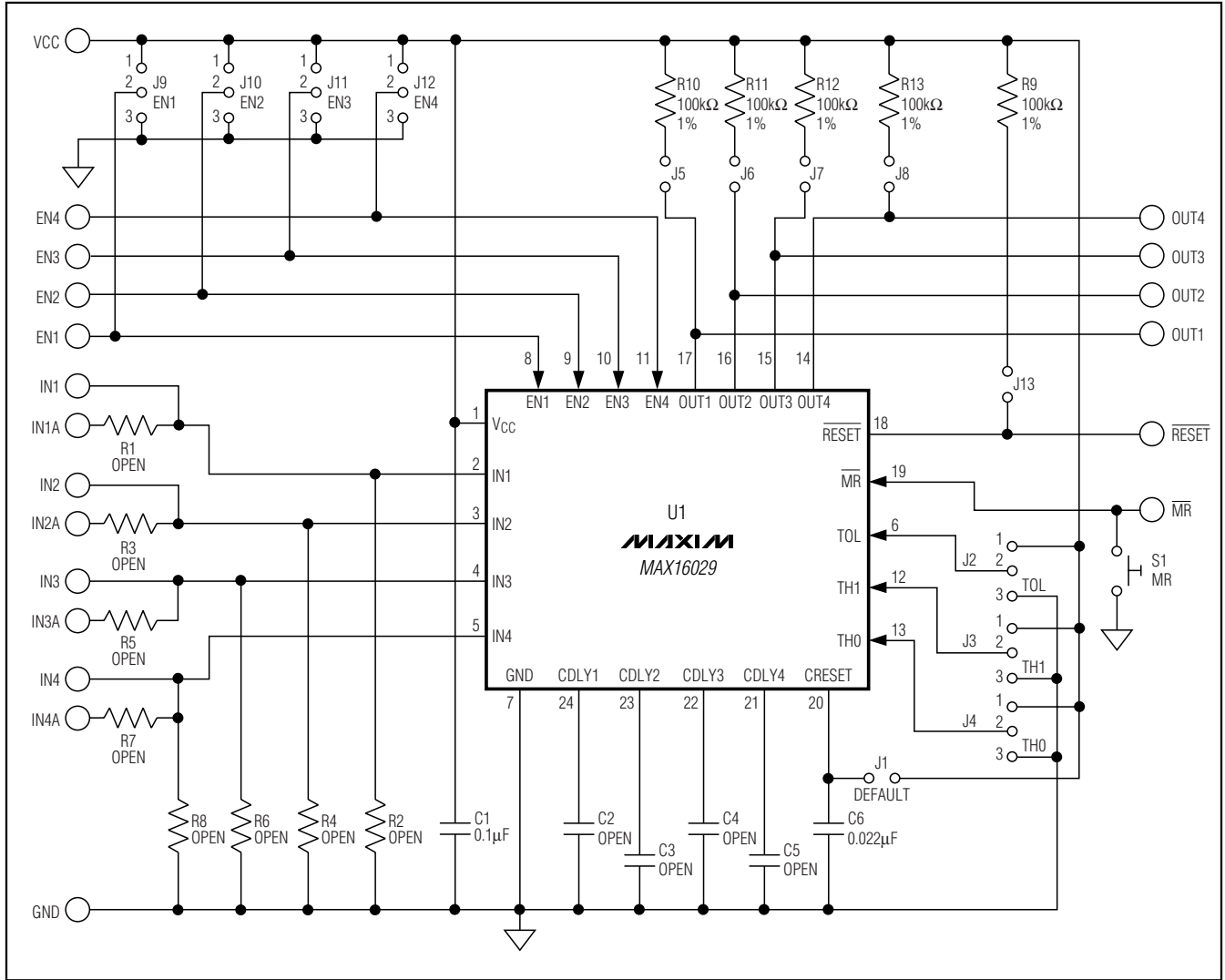
Figure 1. MAX16029EV Kit Schematic
