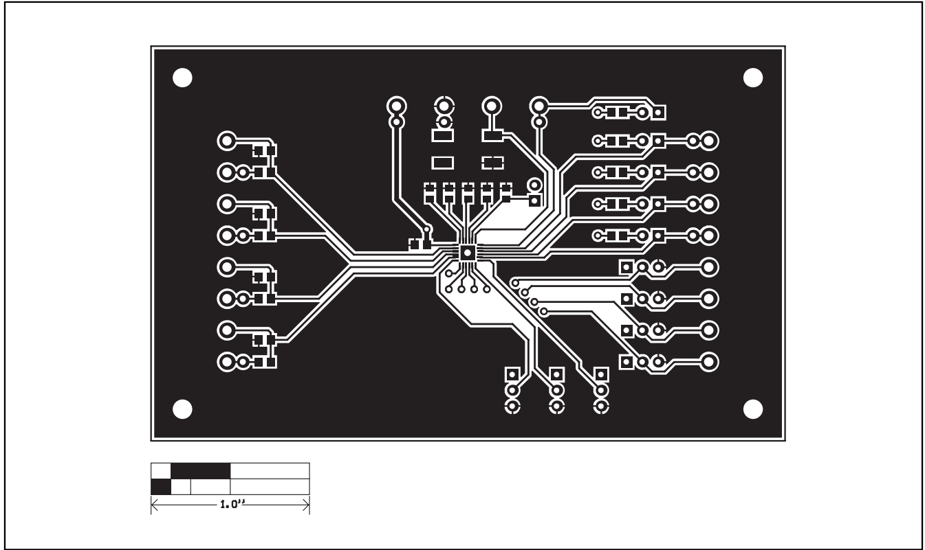
Figure 3. MAX16029EV Kit PCB Layout—Component Side
