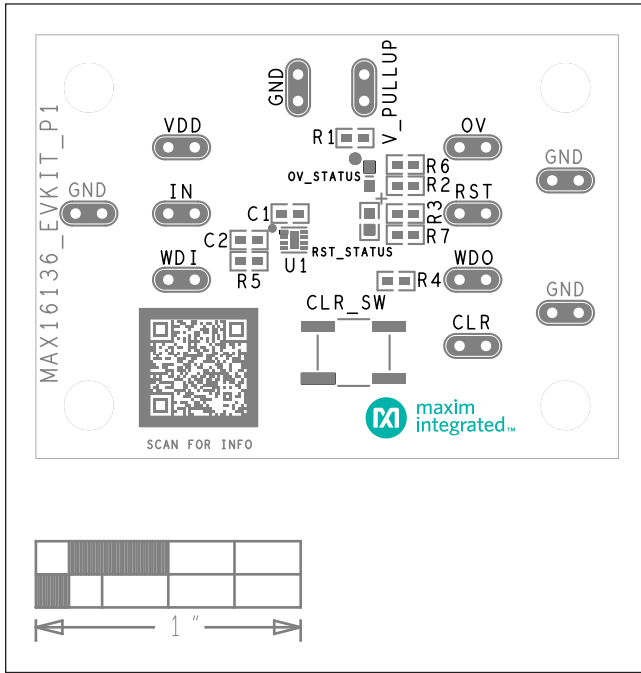
MAX16136 EV Kit PCB Layout—Top Silkscreen
