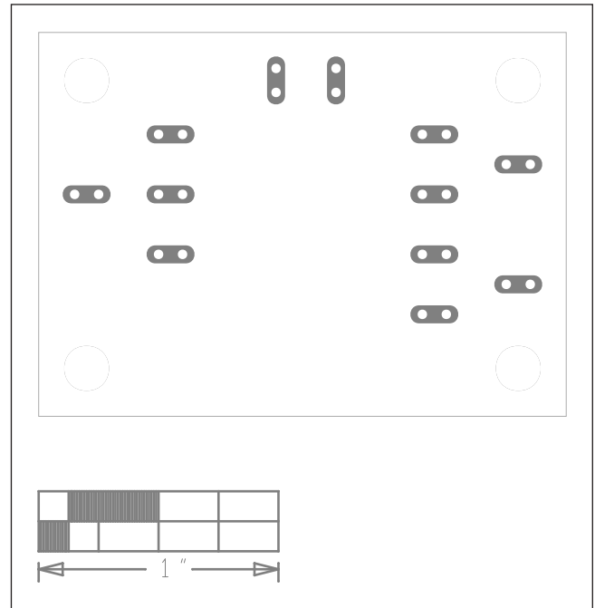
MAX16136 EV Kit PCB Layout—Bottom Silkscreen
