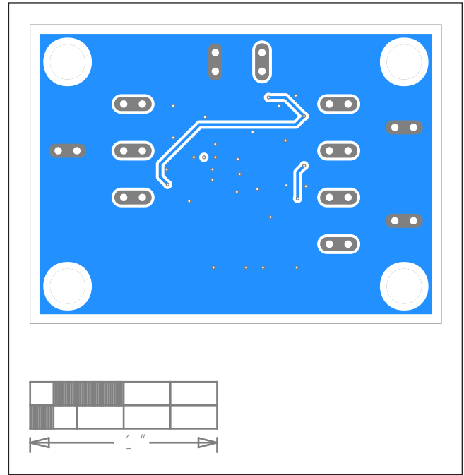
MAX16136 EV Kit PCB Layout—Bottom
