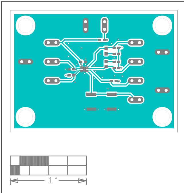
MAX16136 EV Kit PCB Layout—Top
