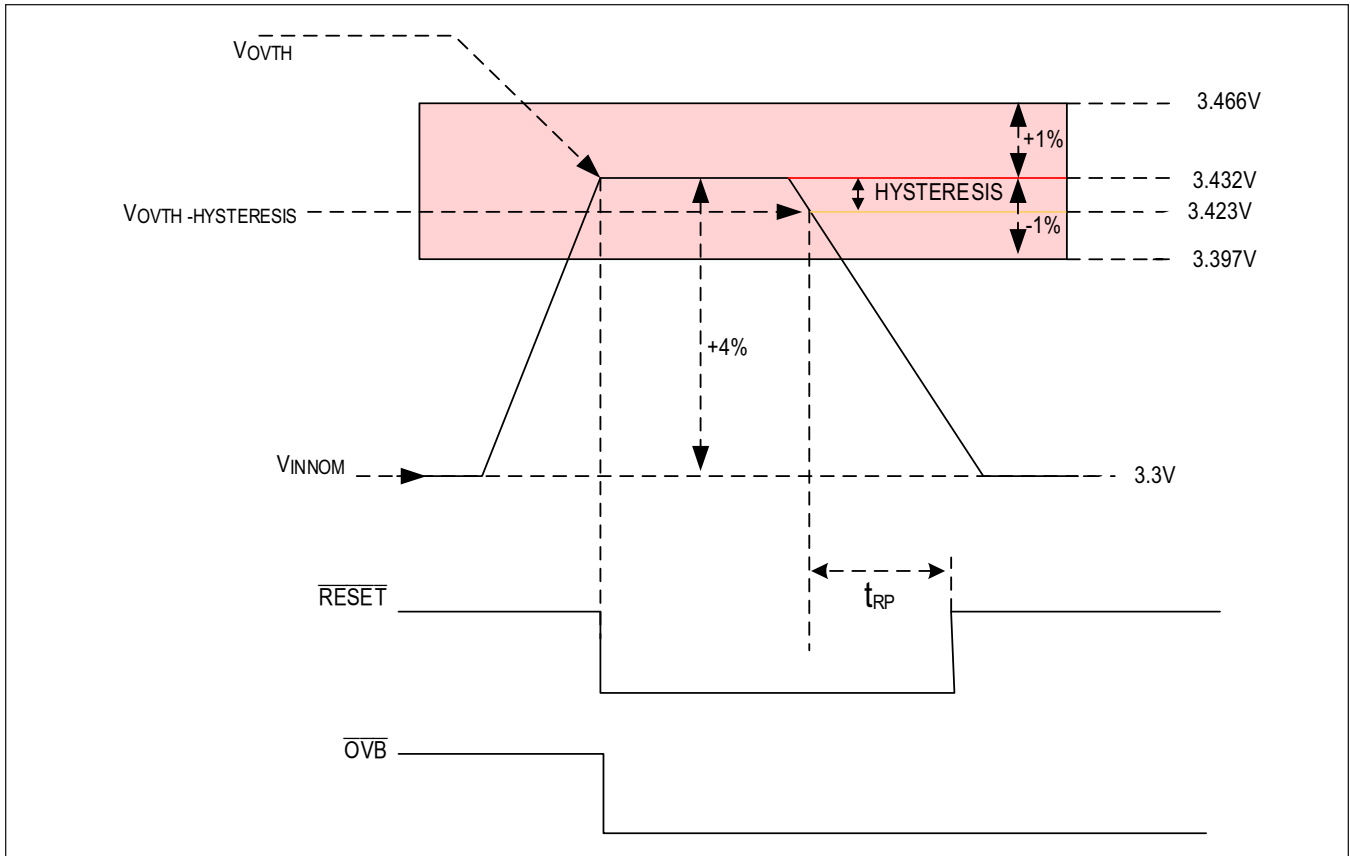
Figure 1: Graphical Description of Overvoltage Threshold
