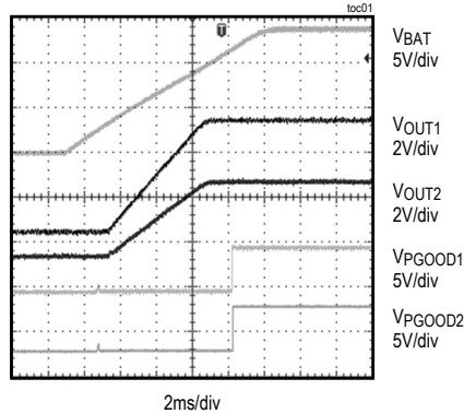
NO LOAD STARTUP SEQUENCE ( V_{FSYNC} = 0\text{V} )
