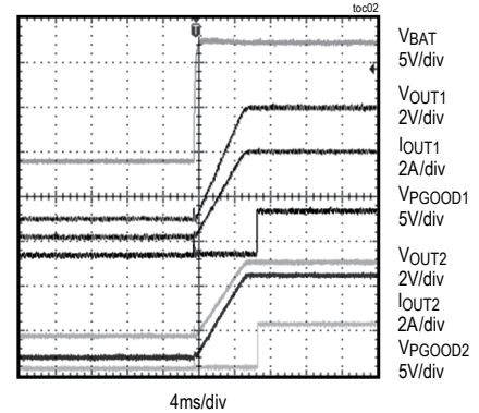
FULL LOAD STARTUP SEQUENCE ( V_{FSYNC} = 0\text{V} )
