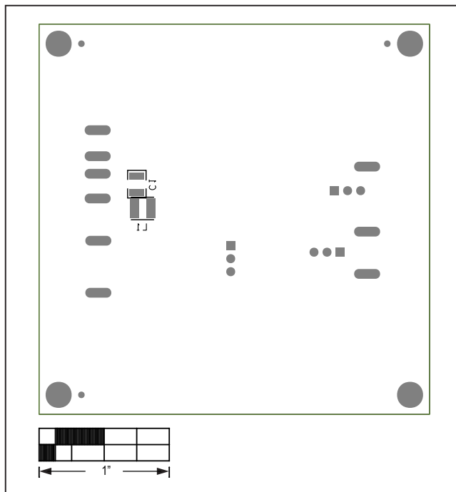
MAX17505EVKITBE# PCB Layout—Bottom Silkscreen
