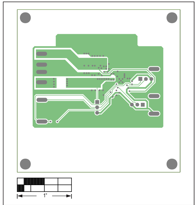
MAX17505EVKITBE# PCB Layout—Layer 3
