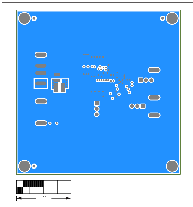
MAX17505EVKITBE# PCB Layout—Bottom Layer
