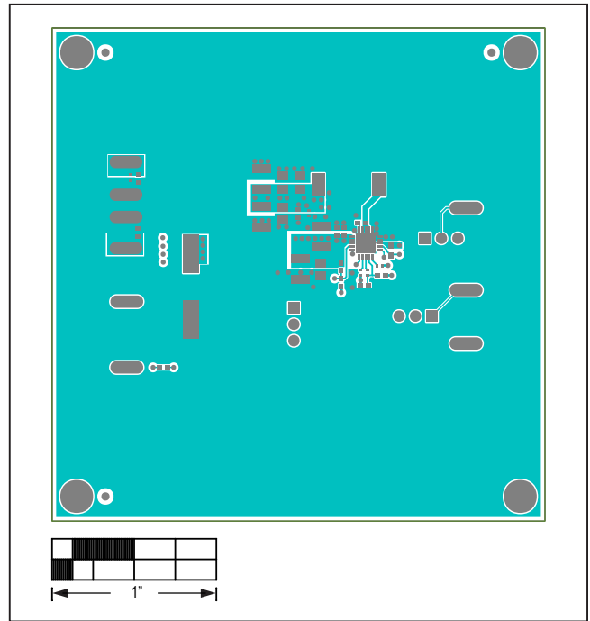
MAX17505EVKITBE# PCB Layout—Top Layer
