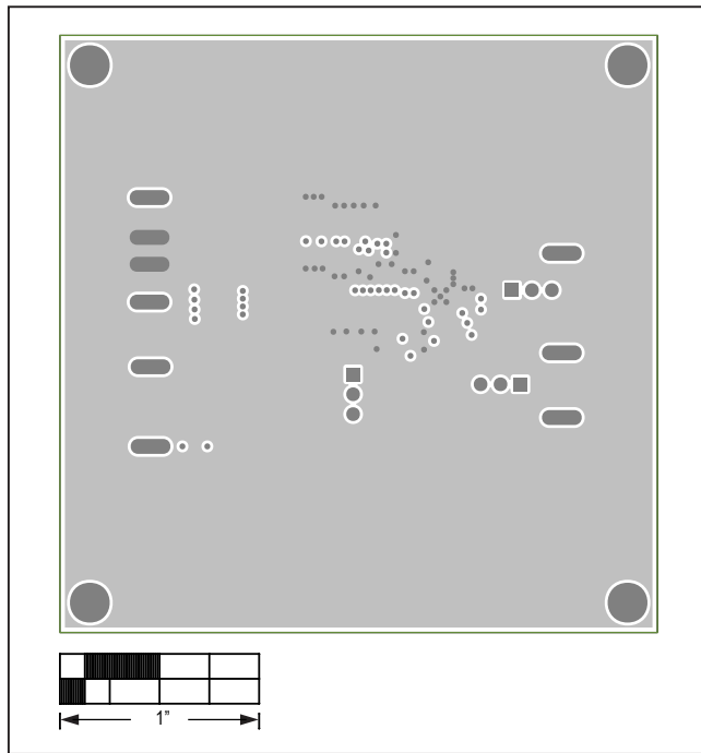
MAX17505EVKITBE# PCB Layout—Layer 2
