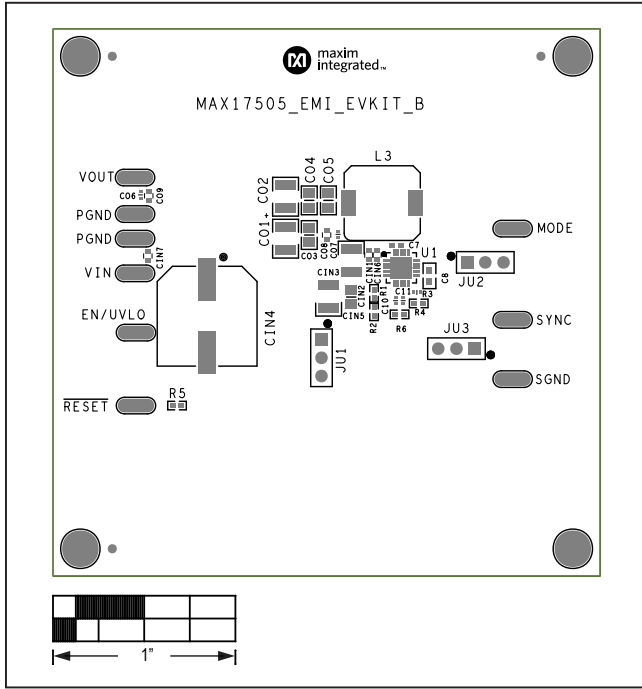
MAX17505EVKITBE# PCB Layout—Top Silkscreen
