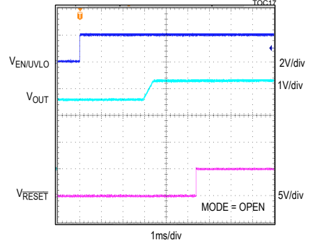
SOFT-START WITH 2.5V PREBIAS, 3.3V OUTPUT, PFM MODE, FIGURE 4B CIRCUIT TOC17
