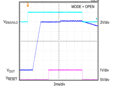
SOFT-START/SHUTDOWN FROM EN/UVLO, 5V OUTPUT, PFM MODE, 5mA LOAD CURRENT, FIGURE 4A CIRCUIT TOC14
