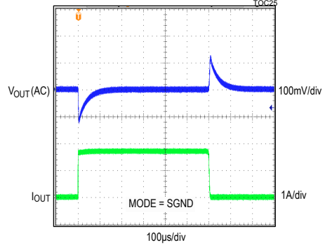
3.3V OUTPUT, PWM MODE, FIGURE 4B CIRCUIT (LOAD CURRENT STEPPED FROM NO LOAD TO 1.75A)
