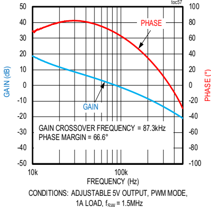
MAX17630C CLOSED-LOOP BODE PLOT FIGURE 7 CIRCUIT
