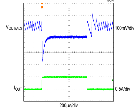
MAX17630B LOAD TRANSIENT BETWEEN 20mA AND 0.5A FIGURE 4 CIRCUIT
