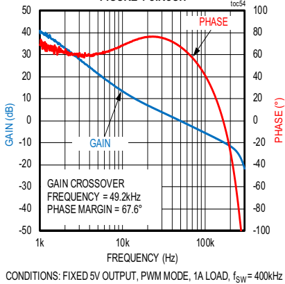
MAX17630B CLOSED-LOOP BODE PLOT FIGURE 4 CIRCUIT
