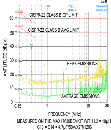
MAX17630B, 5V OUTPUT, 1A LOAD CURRENT CONDUCTED EMI CURVE
