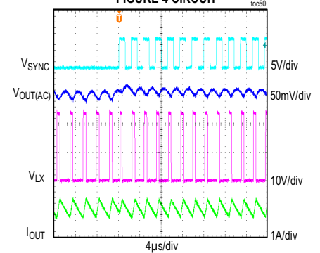
MAX17630B EXTERNAL CLOCK SYNCHRONIZATION FIGURE 4 CIRCUIT
