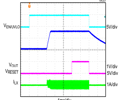
MAX17630A SOFT-START WITH PREBIAS VOLTAGE OF 1.65V FIGURE 3 CIRCUIT toc23
