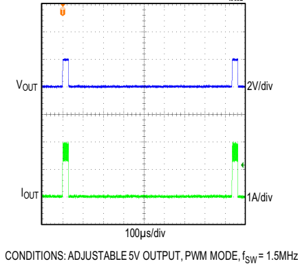
MAX17630C OVERLOAD PROTECTION FIGURE 7 CIRCUIT
