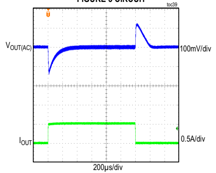
MAX17630A LOAD TRANSIENT BETWEEN 20mA AND 0.5A FIGURE 3 CIRCUIT
