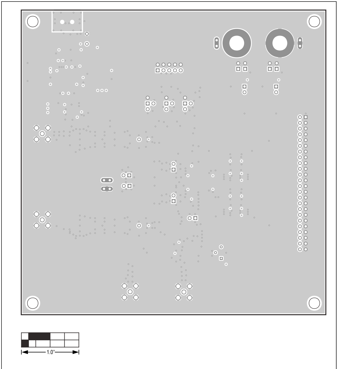
MAX19515/MAX19516/MAX19517 EV Kit PCB Layout—Internal 2
