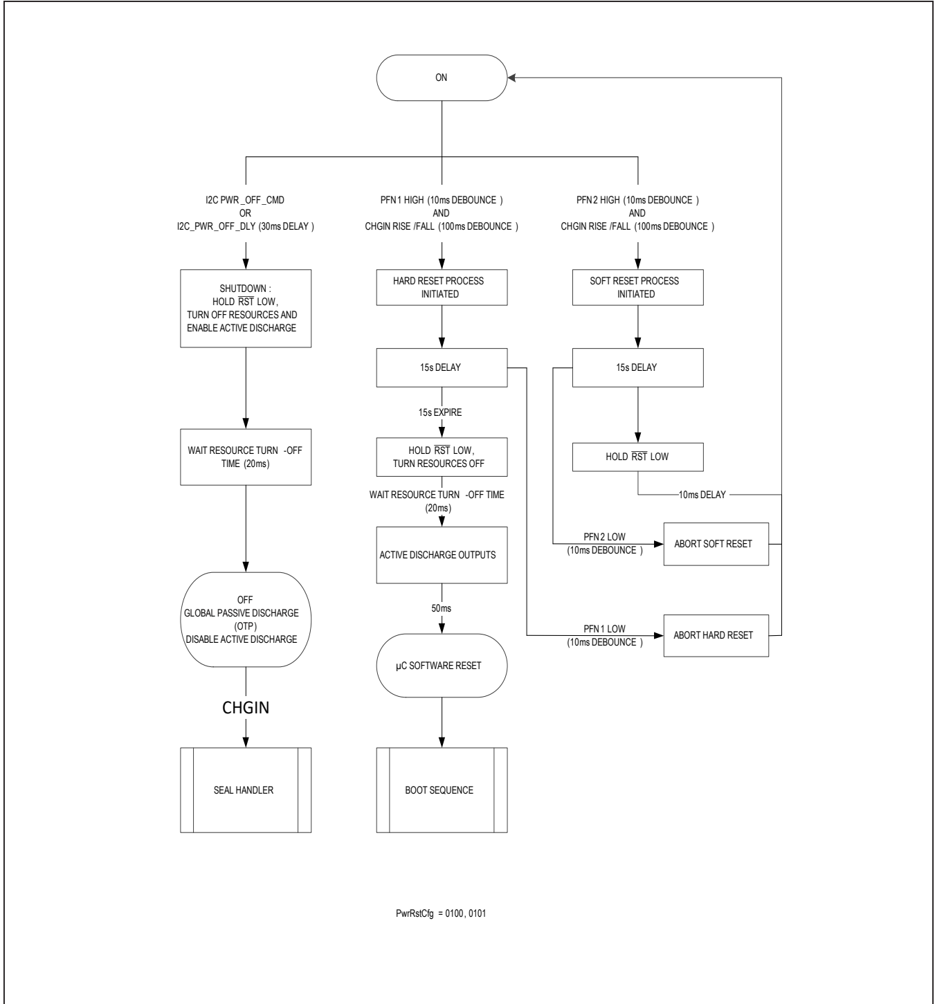
Figure 1c. PwrRstCfg = 0100 or 0101
