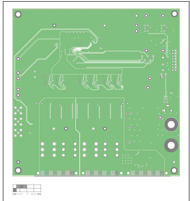
MAX20754 EV Kit---Internal Layer 3 Signal
