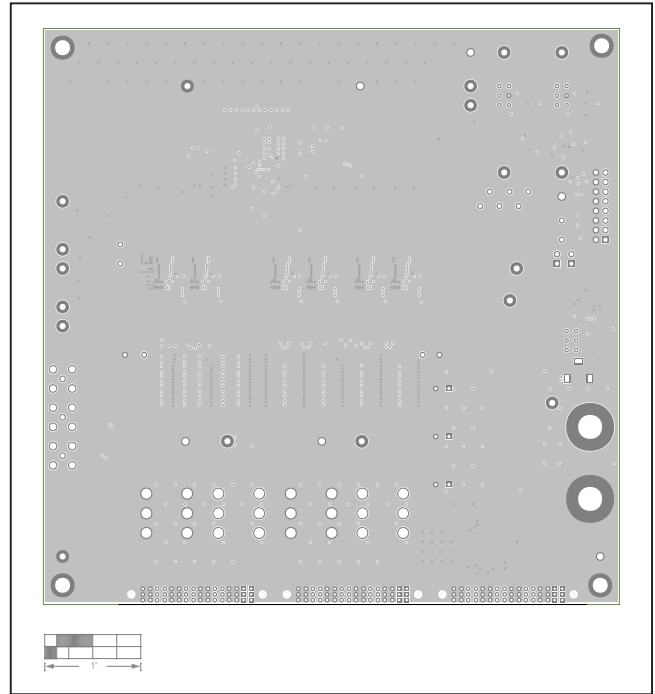
MAX20754 EV Kit---Internal Layer 2 GND
