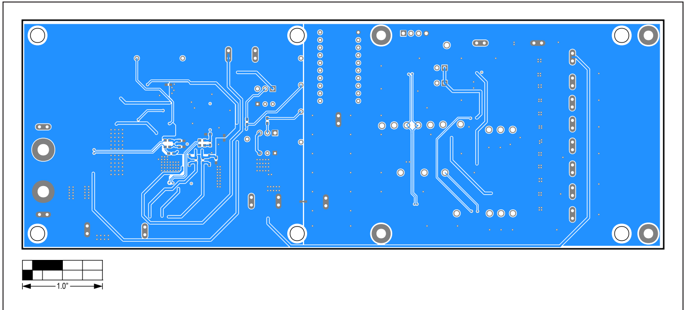
MAX25606 EV System PCB Layout Diagram—Bottom Layer
