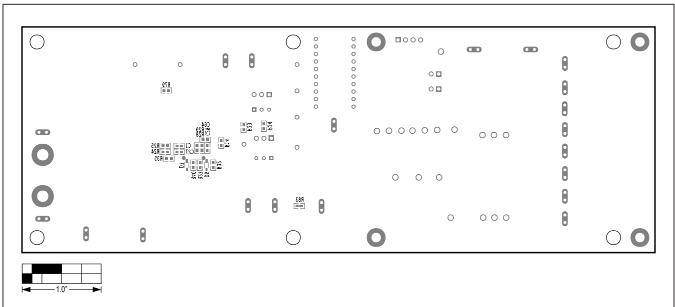
MAX25606 EV System PCB Layout Diagram—Bottom Silkscreen
