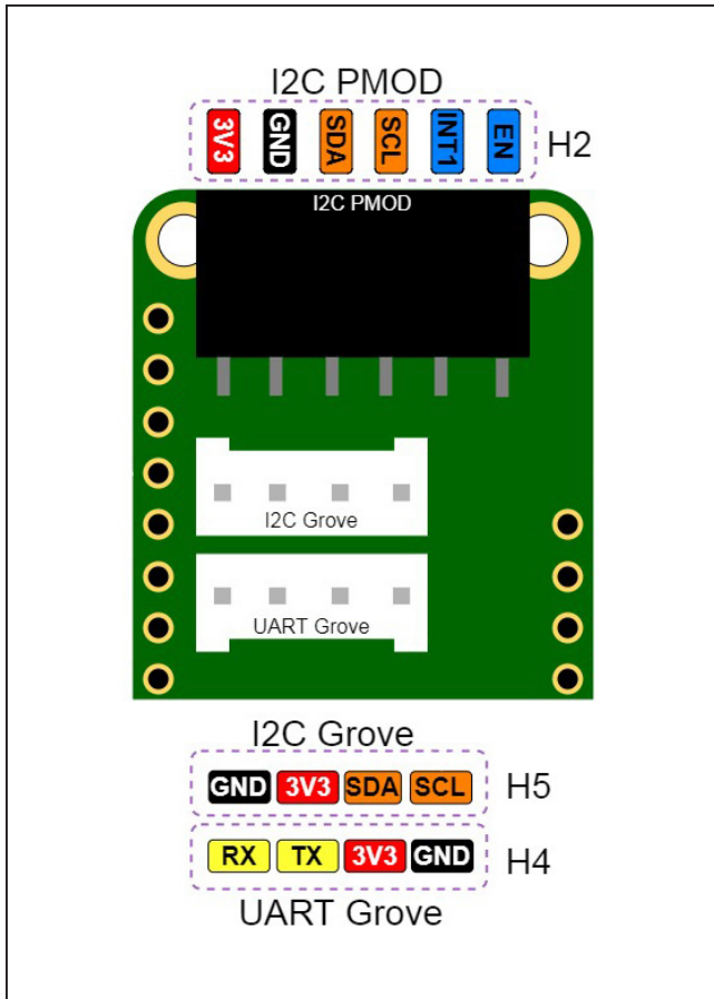
Figure 2. PMOD/Grove Connectors
