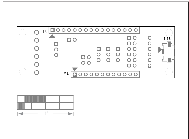
MAX30207EV Interface — Silk Bottom
