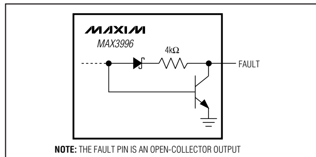
Figure 13. FAULT Output
