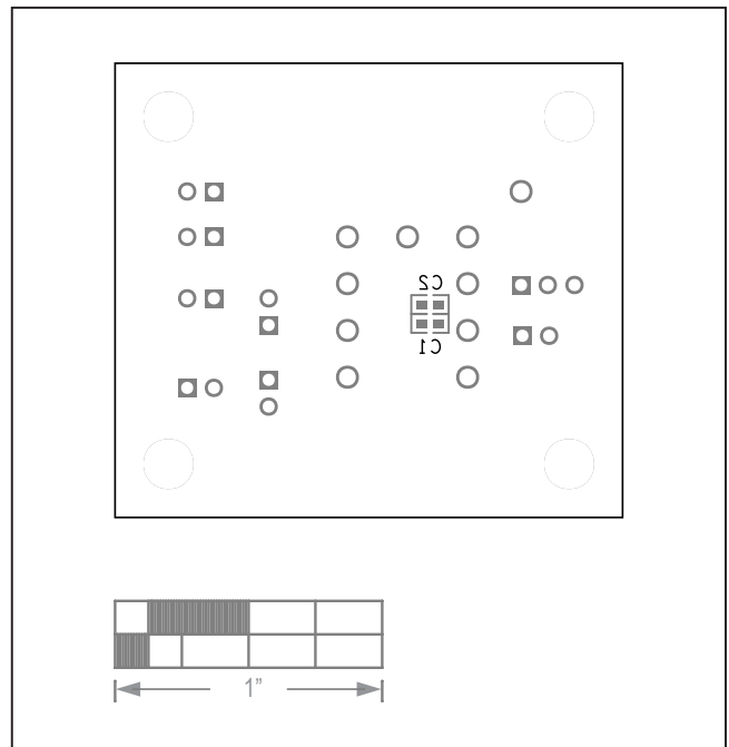
MAX40070 EV Kit PCB Layout—Silk Bottom
