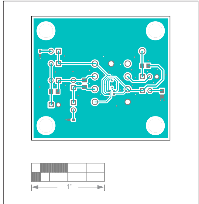
MAX40070 EV Kit PCB Layout—Top
