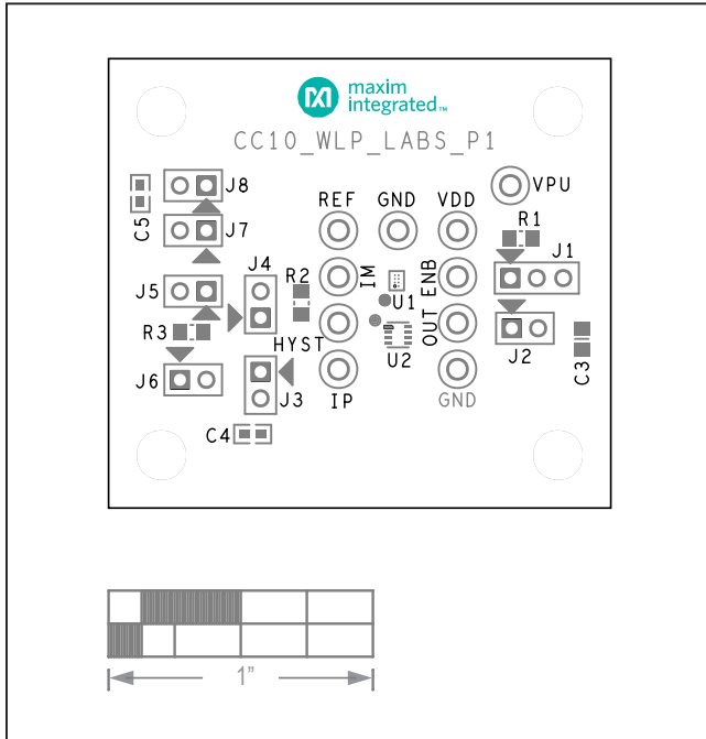
MAX40070 EV Kit PCB Layout—Silk Top
