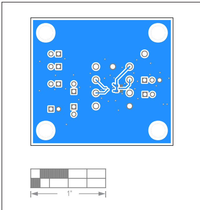
MAX40070 EV Kit PCB Layout—Bottom
