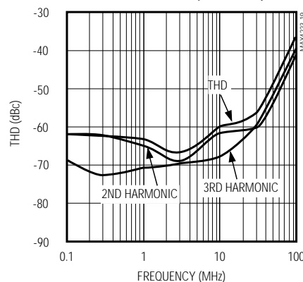
MAX4224/MAX4227/MAX4228 TOTAL HARMONIC DISTORTION vs. FREQUENCY ( R_L = 150\Omega )
