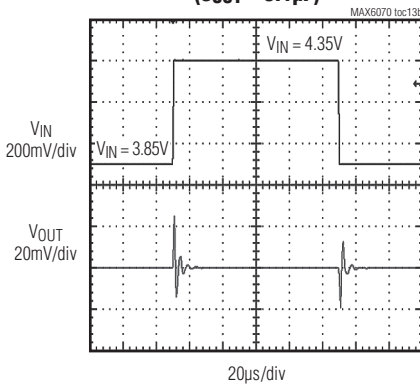
MAX6070_25 LINE TRANSIENT ( C_{OUT} = 0.1\mu\text{F} )
