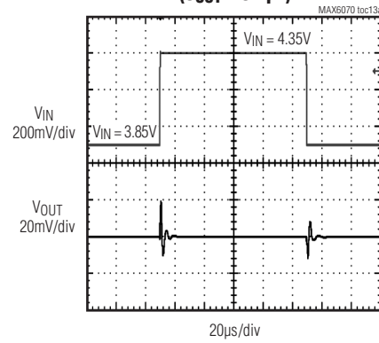
MAX6070_12 LINE TRANSIENT ( C_{OUT} = 0.1\mu\text{F} )
