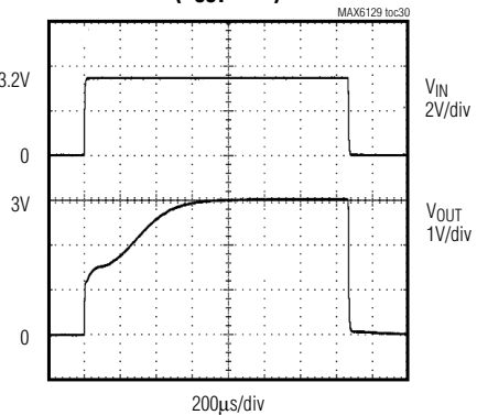
TURN-ON TRANSIENT ( V_{OUT} = 3V )
