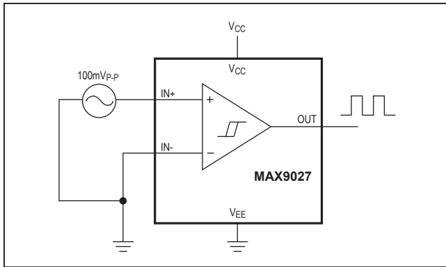
Figure 4. Zero-Crossing Detector
