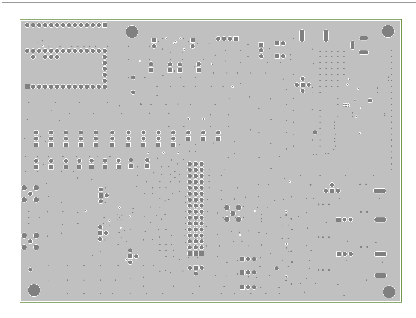
MAX96705A EV Kit PCB Layout—Inner Layer2
