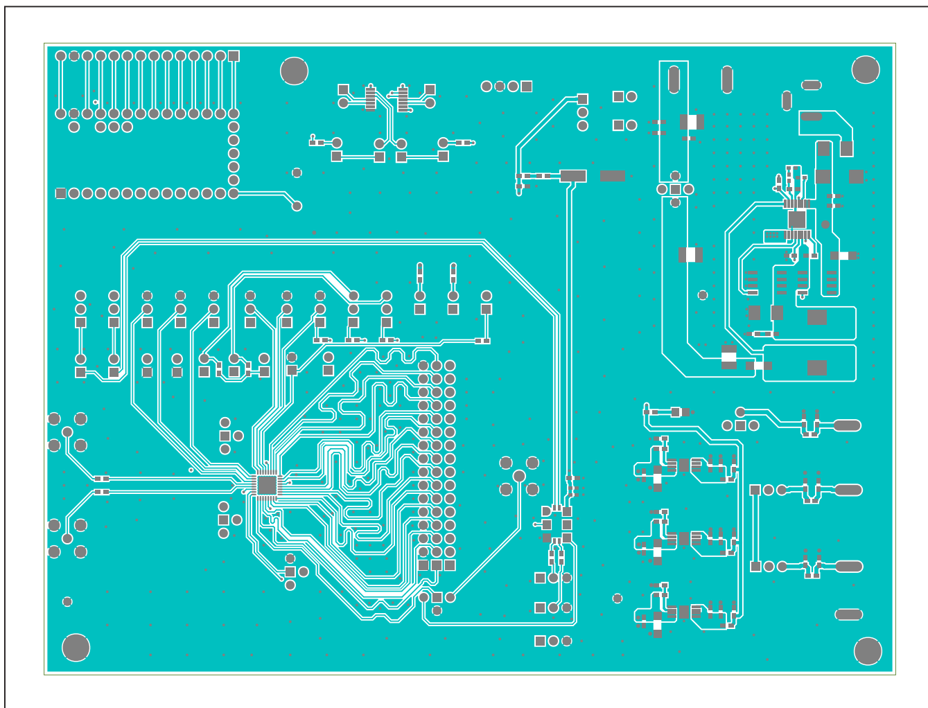
MAX96705A EV Kit PCB Layout—Top Layer
