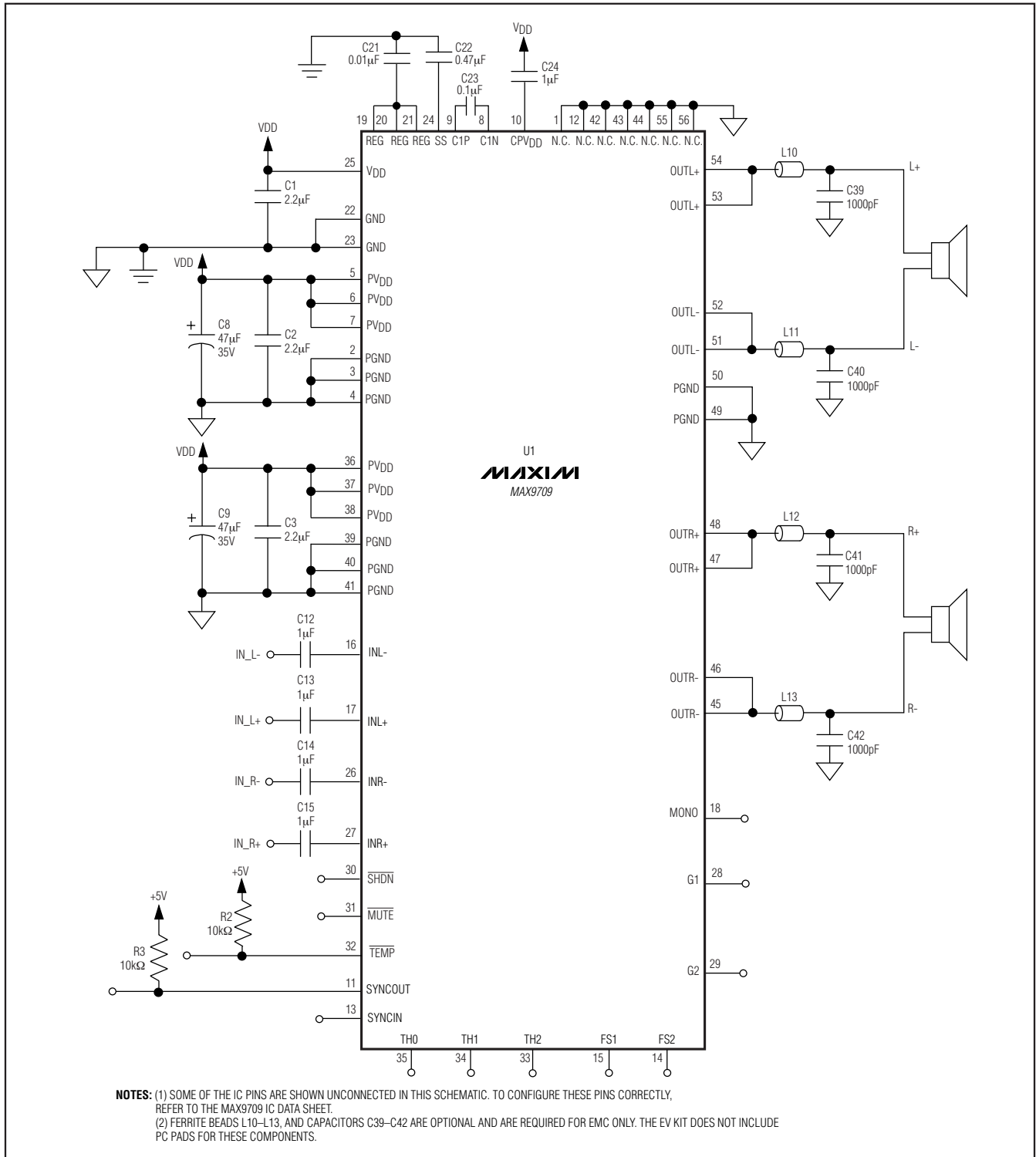
Figure 1. MAX9709 Customer Design Schematic with Minimal Components
