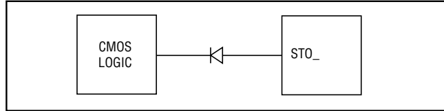
Figure 3. Driving STO_ with CMOS Logic
