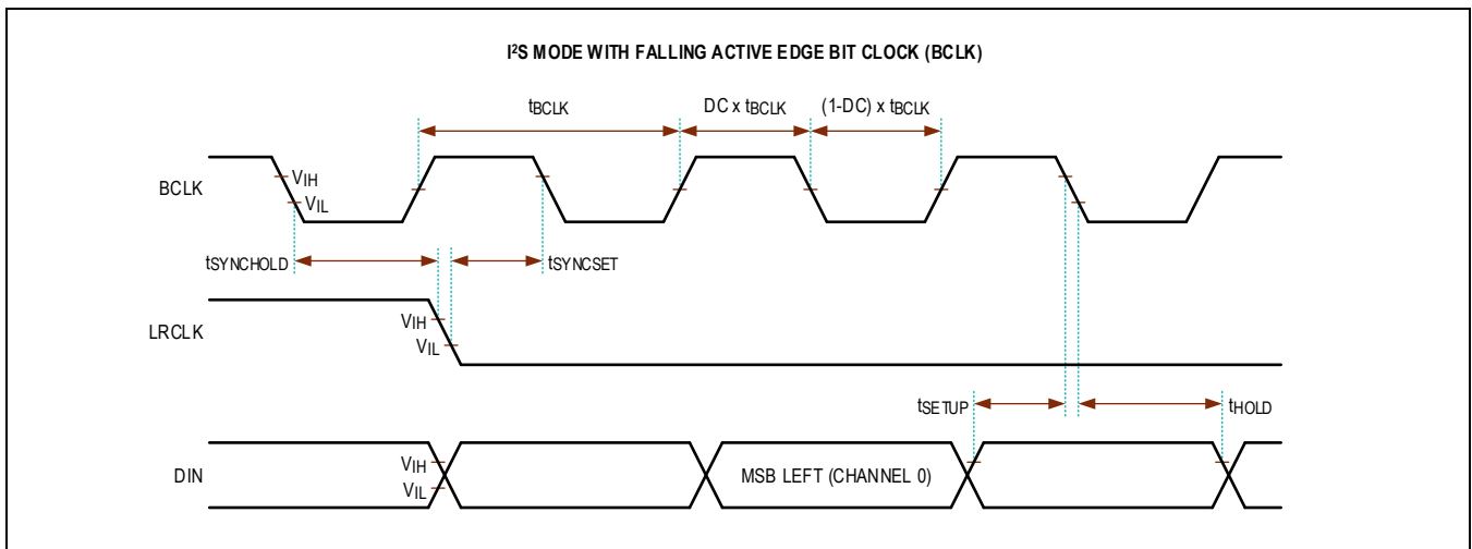
Figure 2. PCM Interface Timing Diagram for I²S Mode
